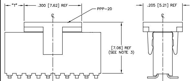
"R" = USE MEASURED DIMENSION (REF) "T" = {("R" - .300)/2} ±.020
